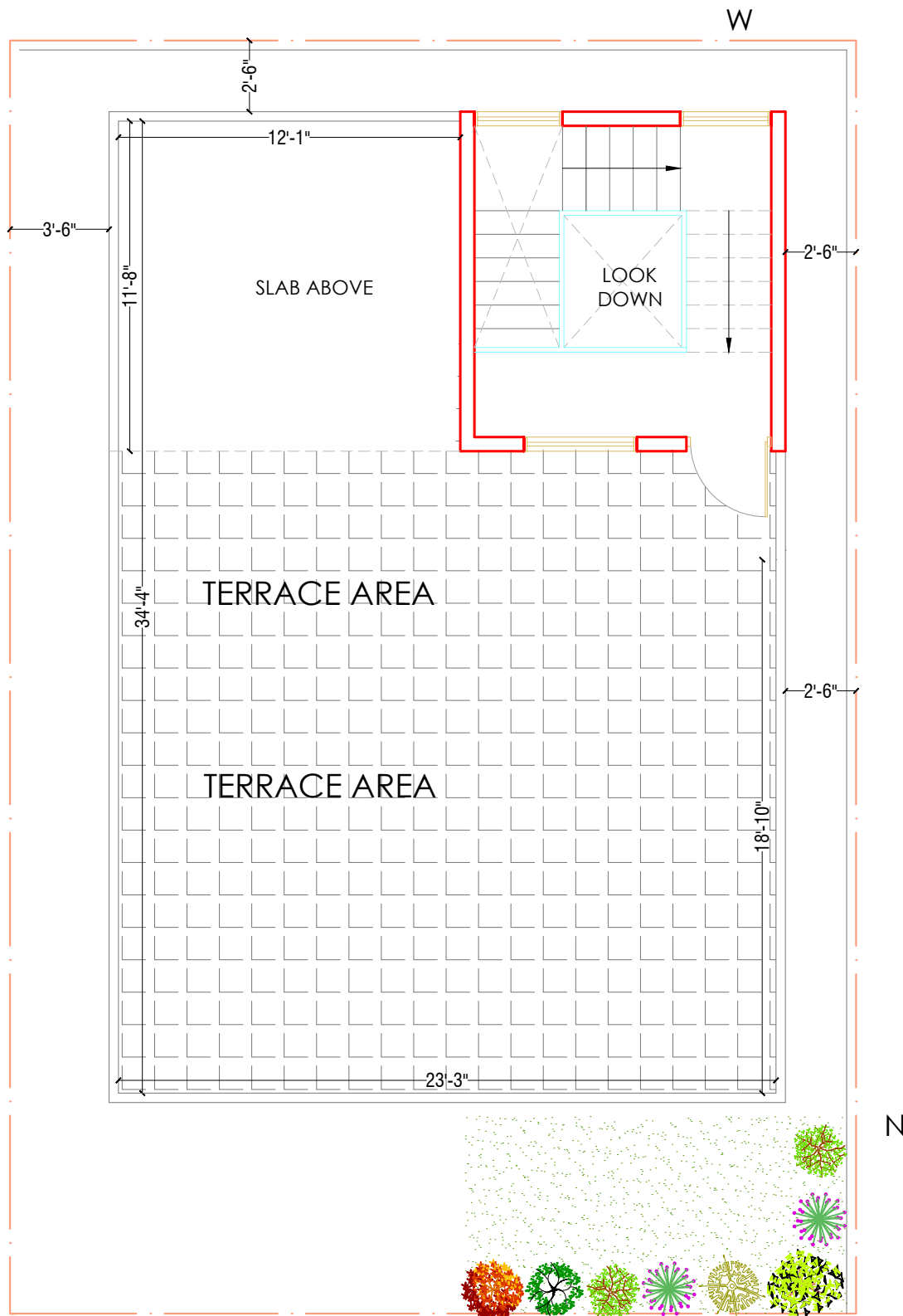
2 nd TERRACE FLOOR PLAN :- 138 SFT additional slab projection :- 150 sft
